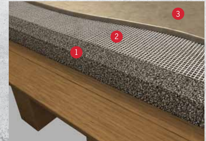
1 ARDEX LS 2 ARDEX BU-R 3 ARDEX K 71
